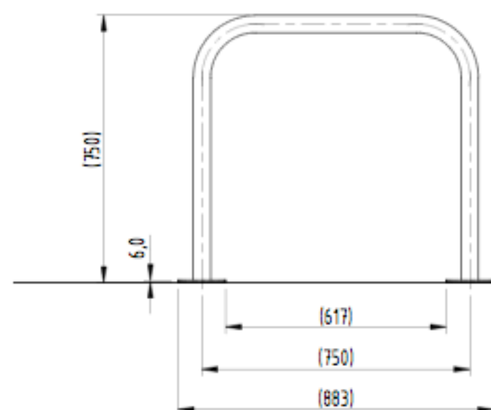
138200101 - FLANGED VERSION
