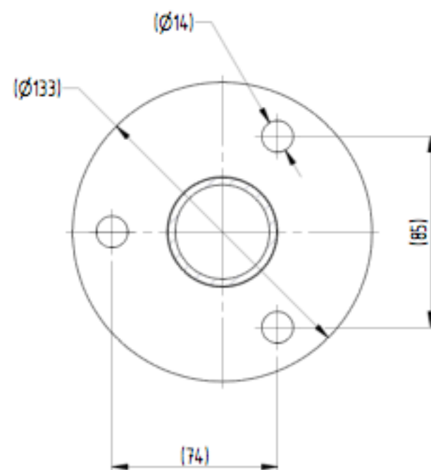
SHEFFIELD FLANGE PLATE DIMENSIONS
