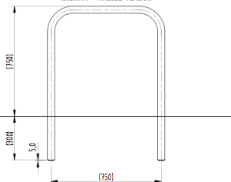
138200111 - RAGGED VERSION
