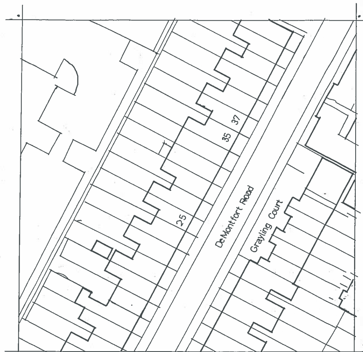
Block plan 1:500
