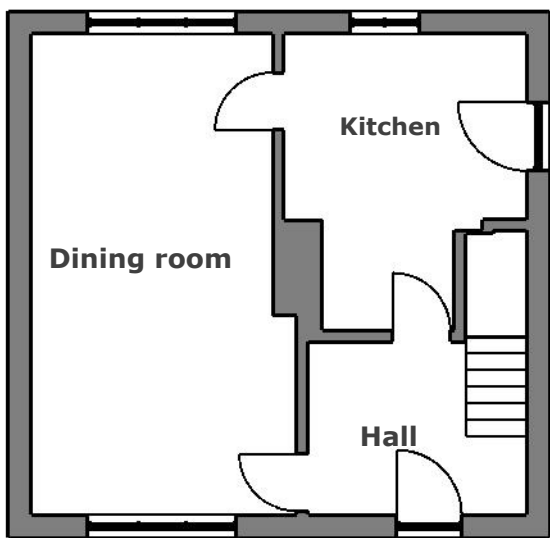
Existing ground floor plan 1:100
