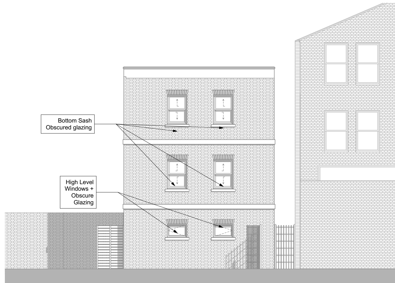
E-03 Rear Elevation 1:100
