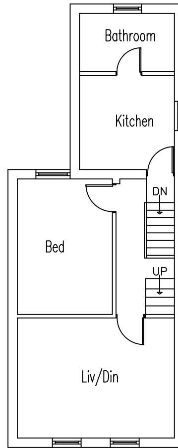
First Floor No. 28-A Norfolk Road
