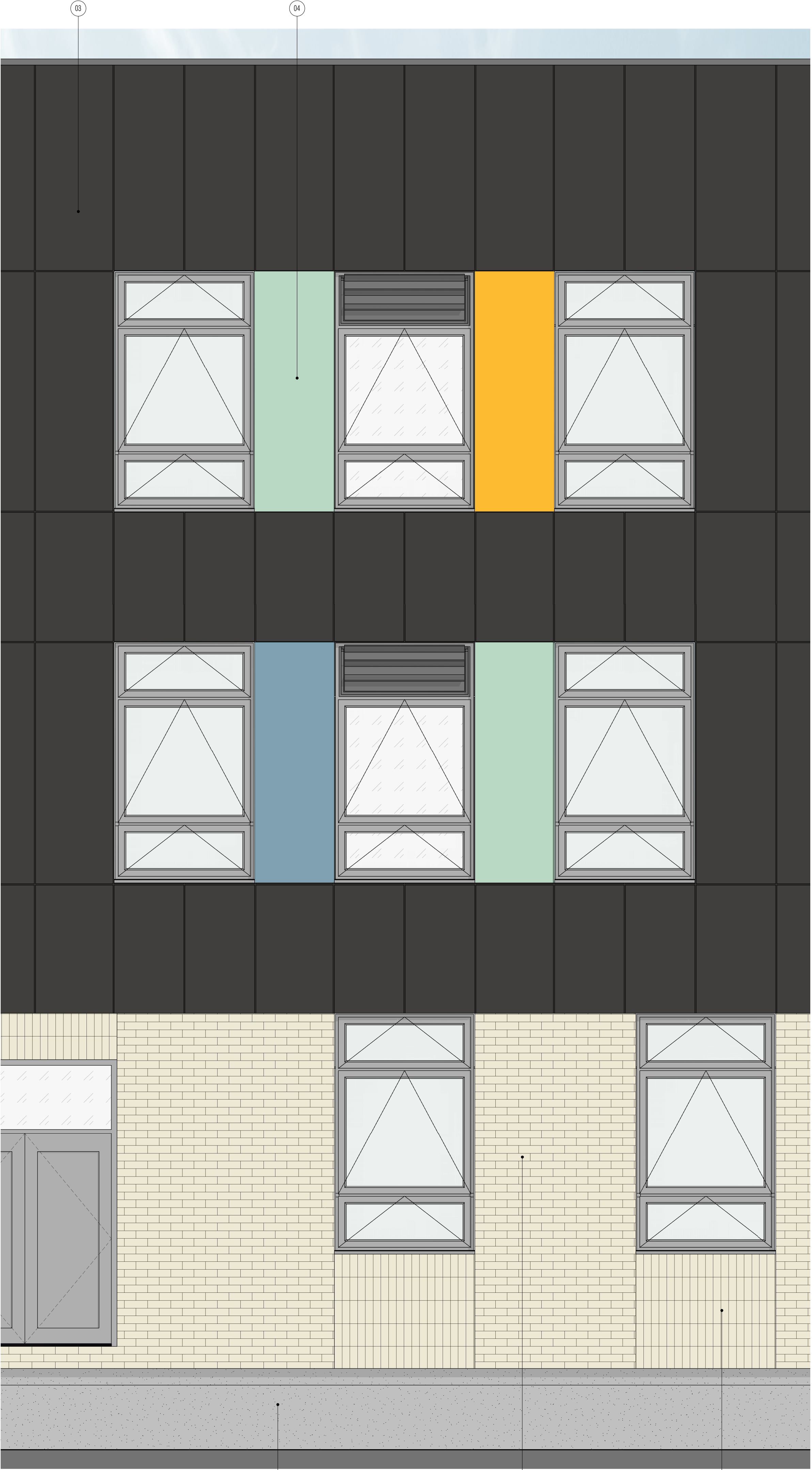
1 Enlarged Bay Elevation - Typical Teaching Wing 3010 1:25
