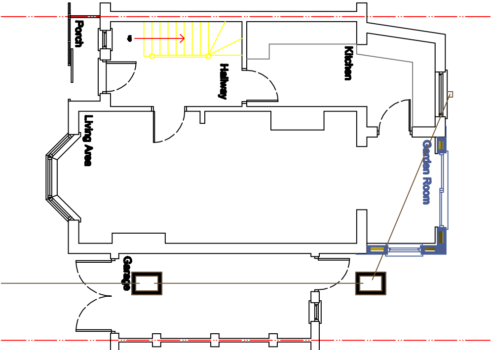
54 Buxton Avenue Ground Floor Plan Gross Internal = 69.00sq.m.
