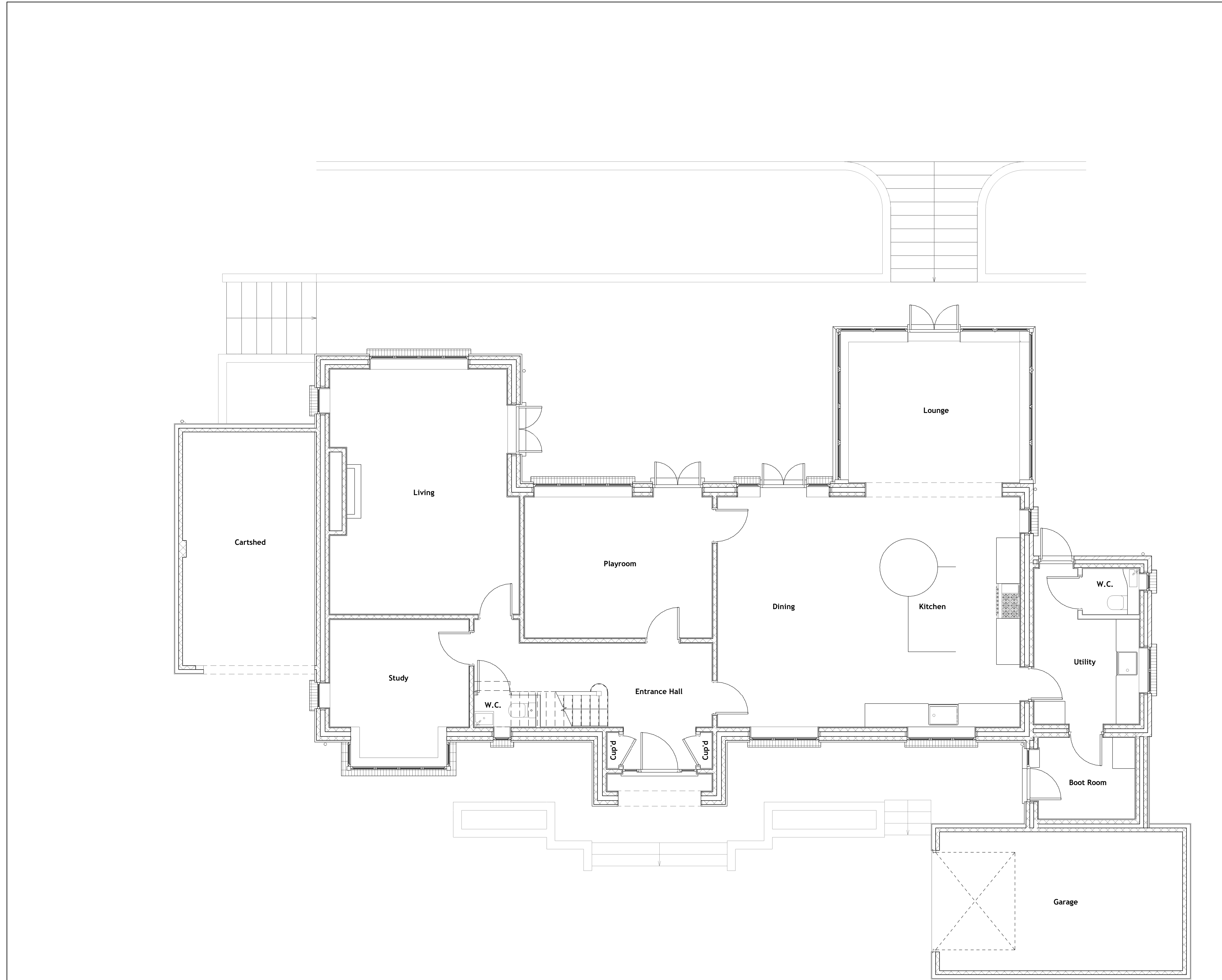
Existing Ground Level Plan General Arrangement | 00-FFL | Scale 1 : 50
