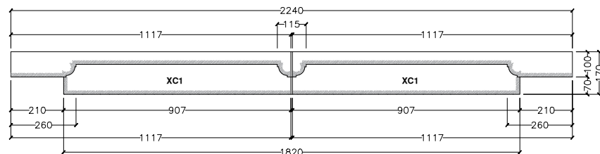
XC1 Stooled Cill Plan
