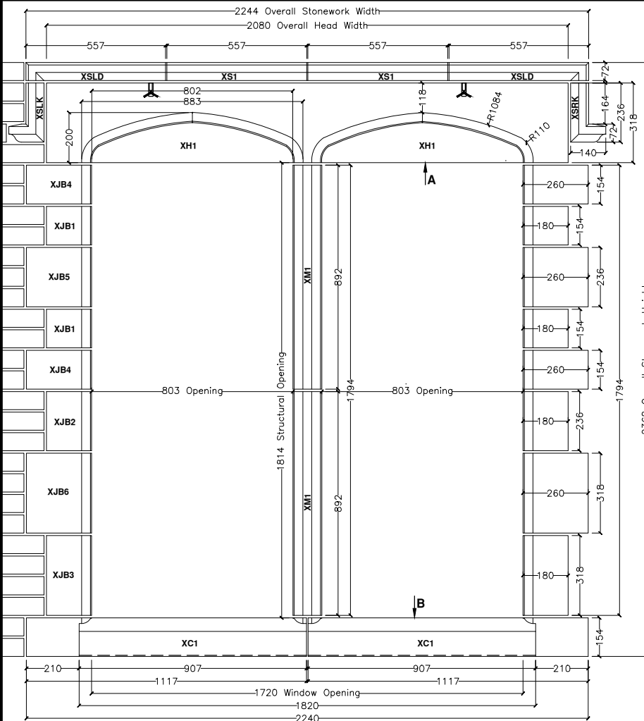
Window Surround Elevation
