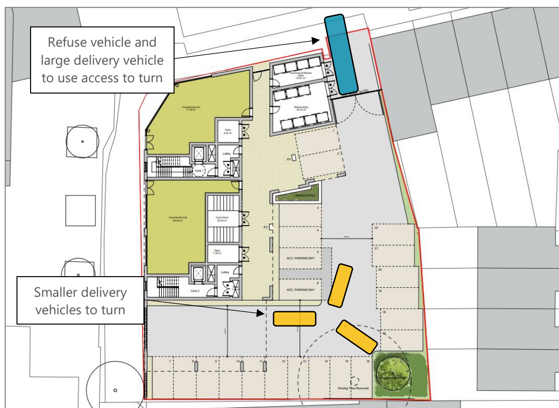
Image 3.2: Site Servicing Arrangements
