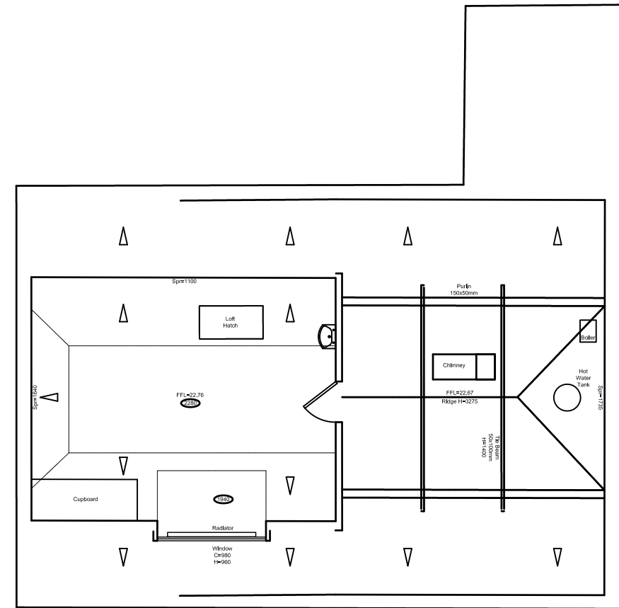
EXISTING LOFT PLAN
