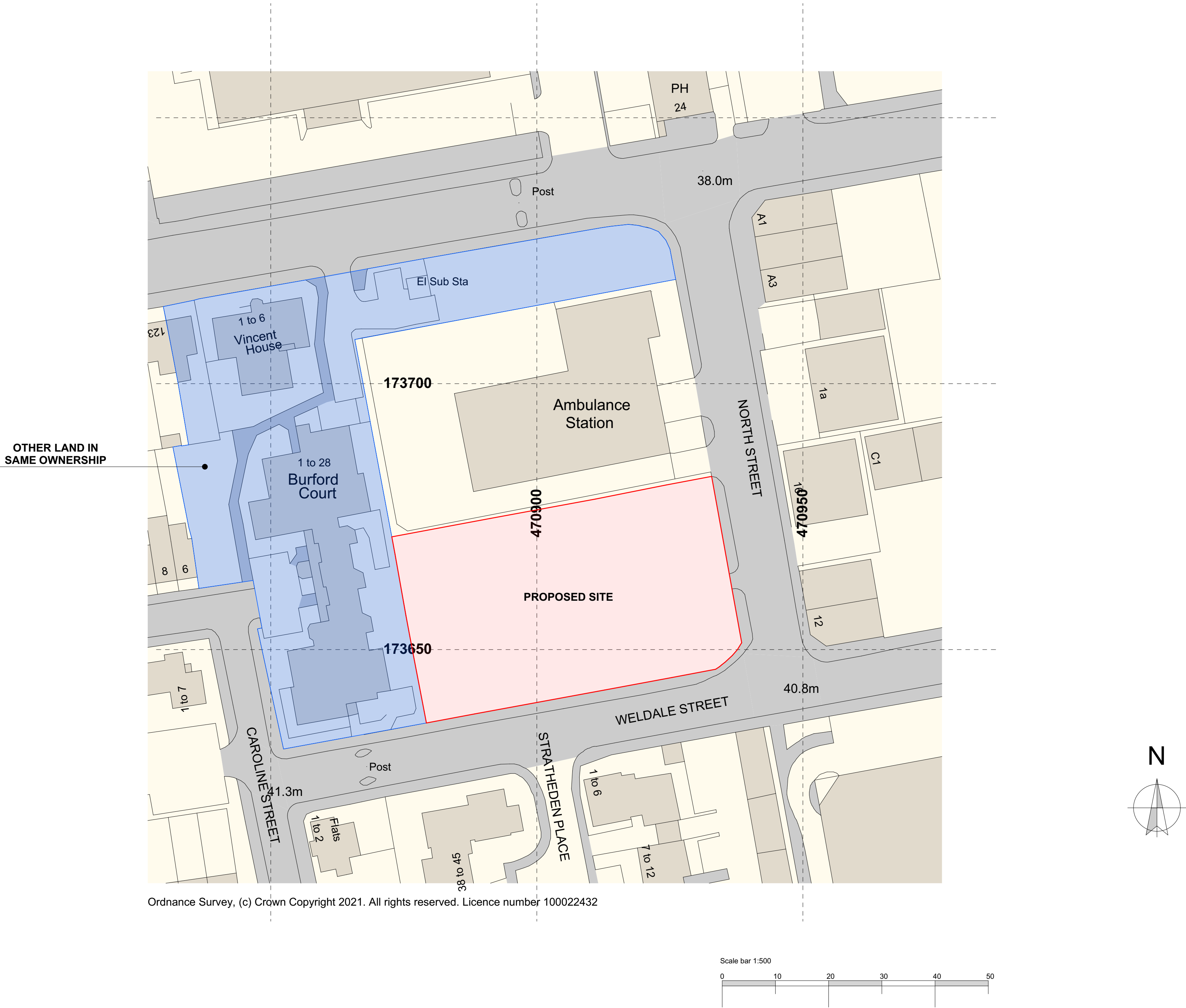
SITE BLOCK PLAN - 1:500 SCALE
