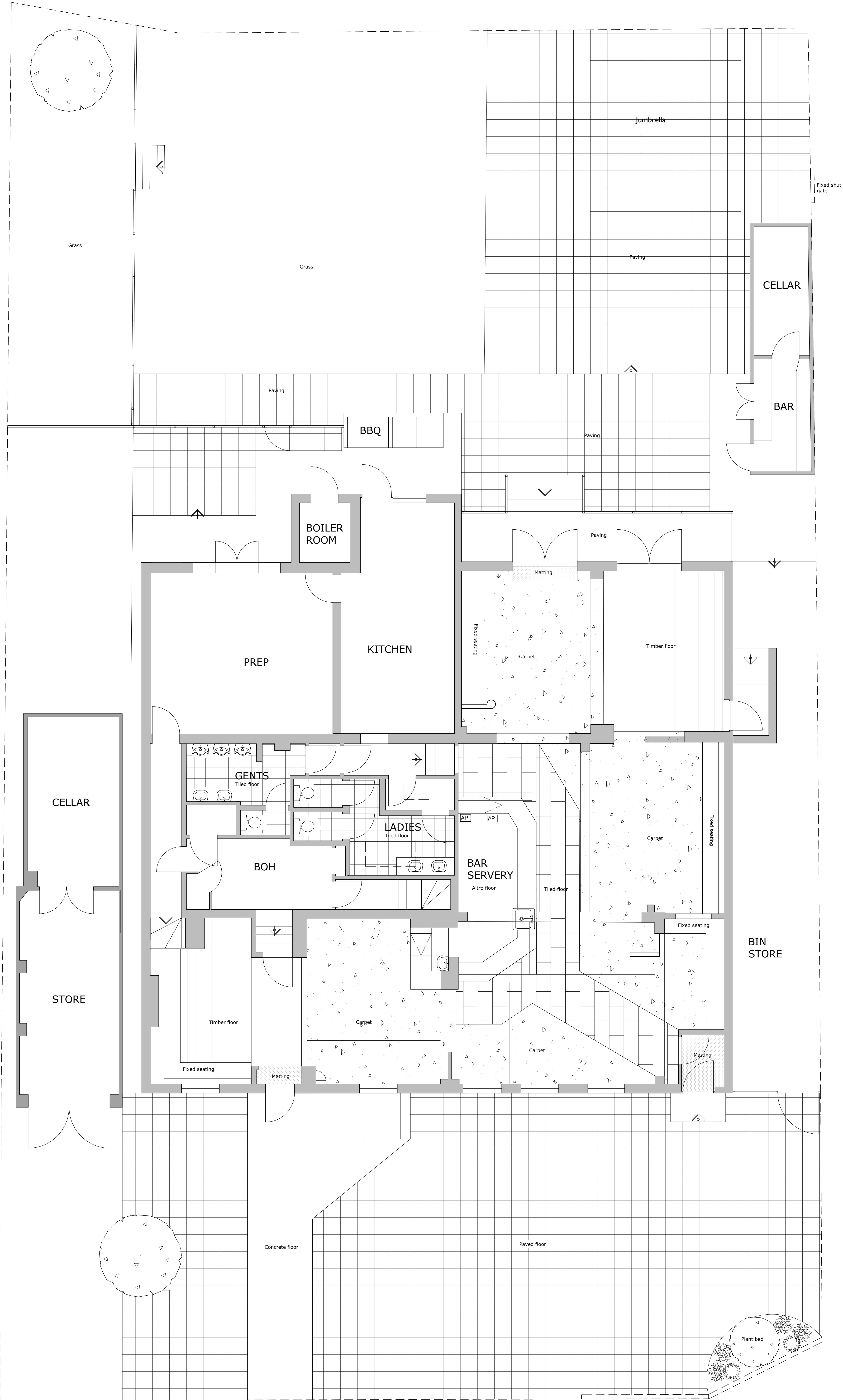
Existing ground floor plan
