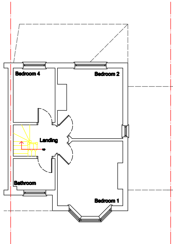
54 Buxton Avenue First Floor Plan Gross Internal = 43.50sq.m.
