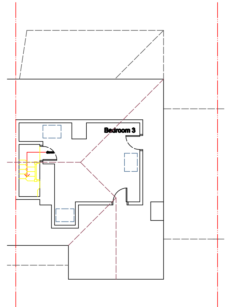
54 Buxton Avenue Attic Floor Plan Gross Internal = 17.50sq.m.
