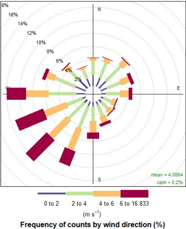
Figure 2 Windrose for Heathrow 2016-2020
