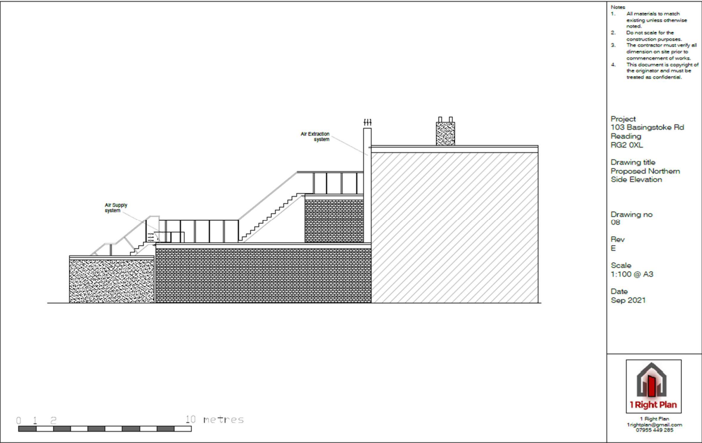
Figure 4 Proposed side elevation (Source 1 Right Plan)
