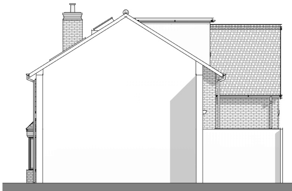
5 East Elevation_Northfield Road 1 : 100
