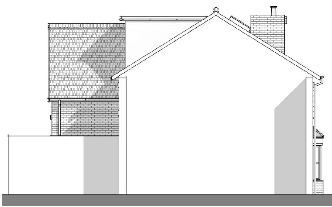
1 North Elevation_Swansea Road 1 : 100
