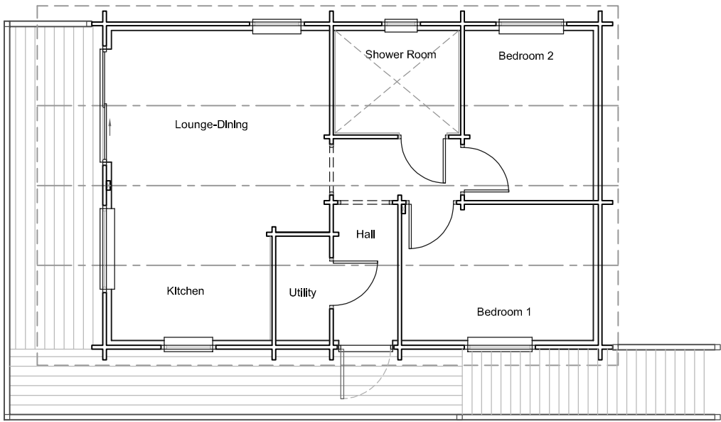
Floor Plan
