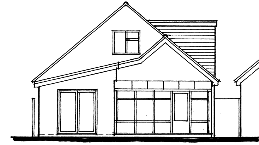
rear elevation
