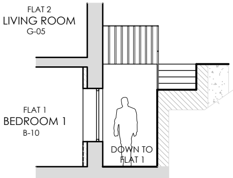
PROPOSED SECTION 6-6 1:100
