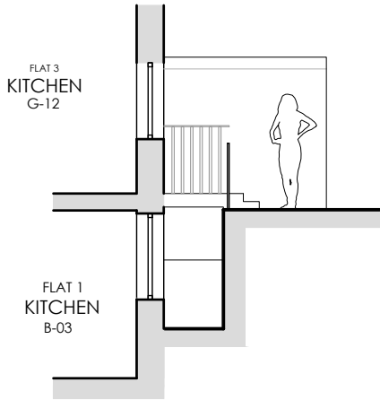
PROPOSED SECTION 3-3 1:100
