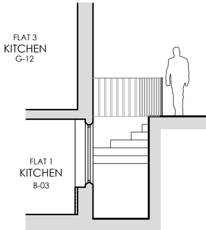
PROPOSED SECTION 4-4 1:100
