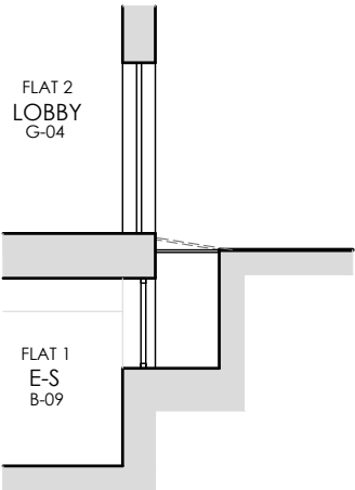
PROPOSED SECTION 7-7 1:100
