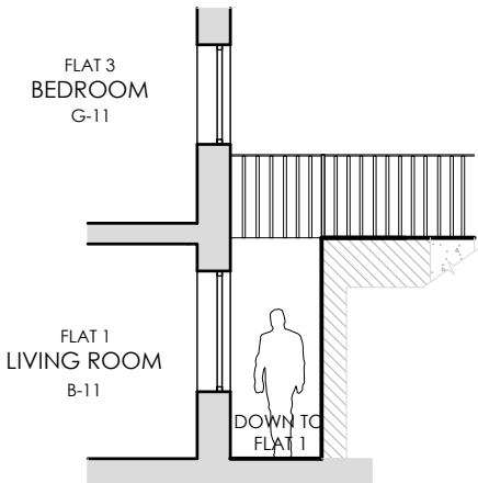
PROPOSED SECTION 5-5 1:100
