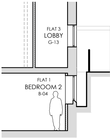
PROPOSED SECTION 2-2 1:100
