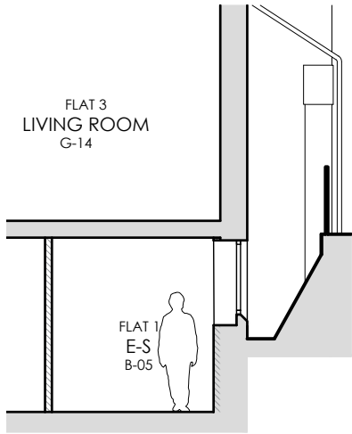
PROPOSED SECTION 1-1 1:100
