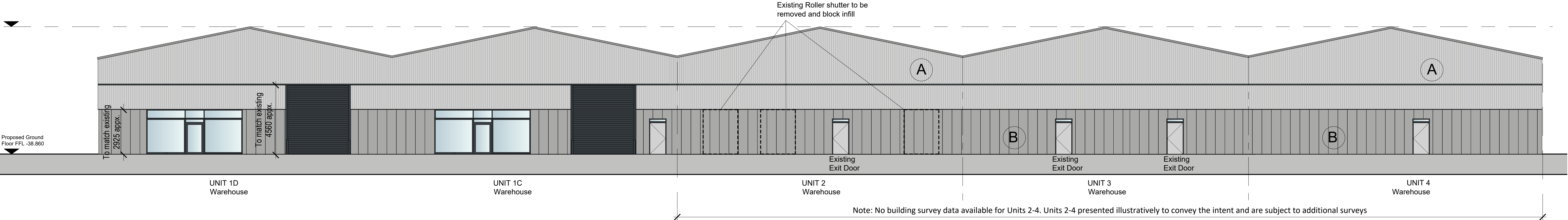
NORTH-WEST ELEVATION
