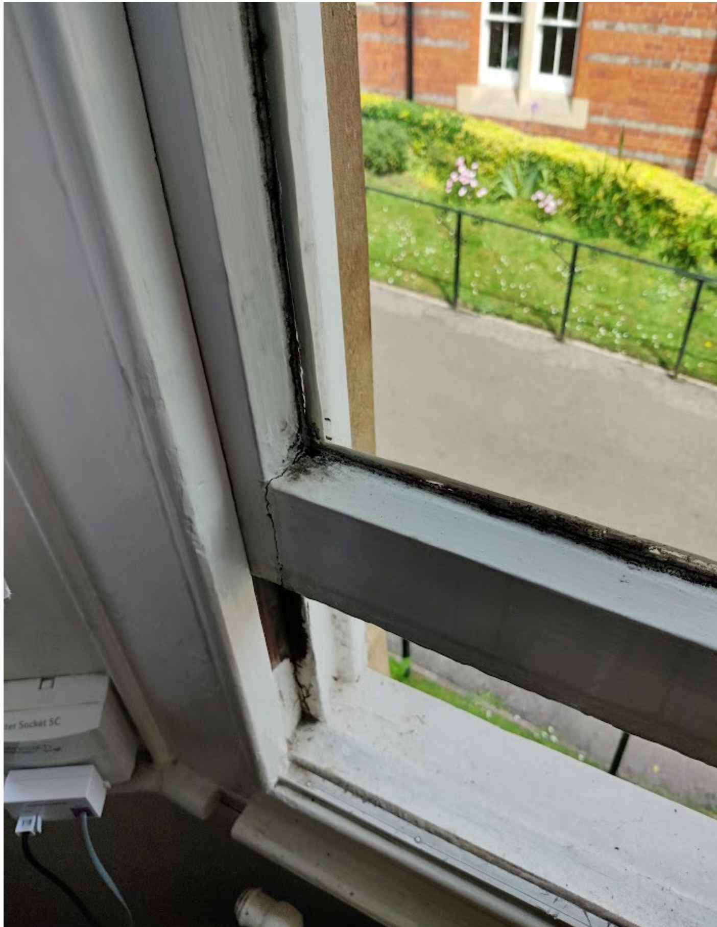
Figure 9. Typical Joint Opening Up in Lower Sash Frame
