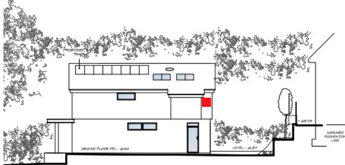
SOUTH EAST ELEVATION - PLOT 1
