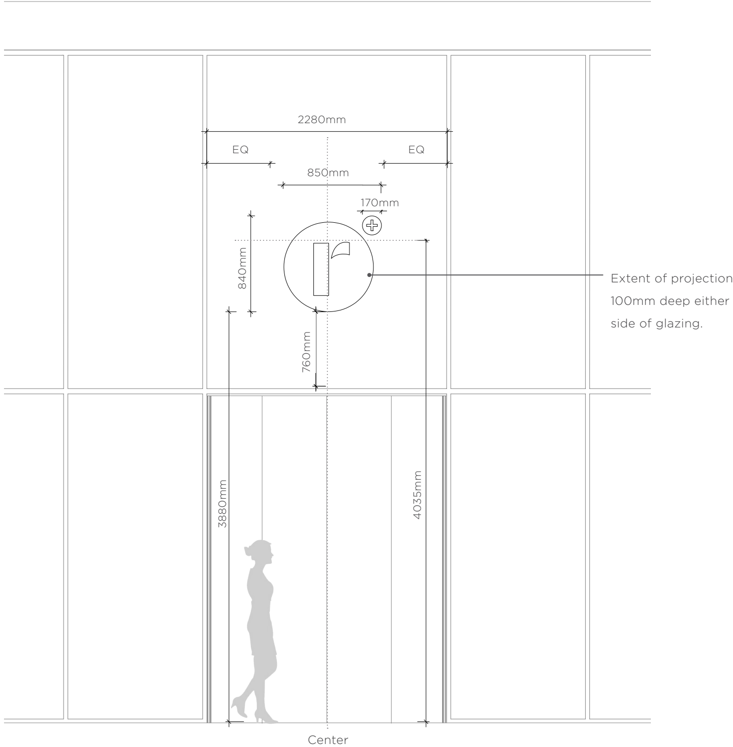
Front Entrance Elevation
