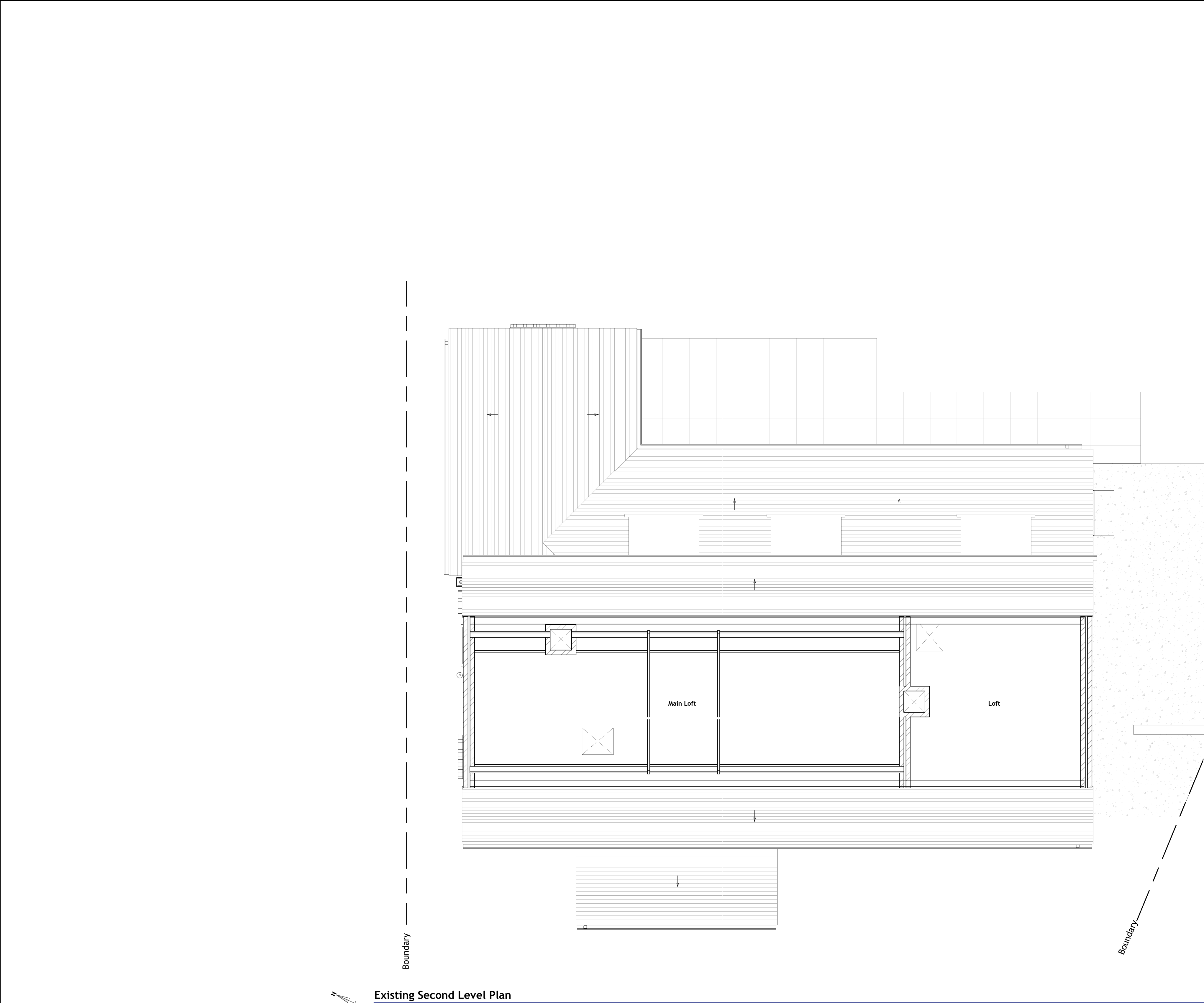
Existing Second Level Plan General Arrangement | 02-FFL | Scale 1 : 50
