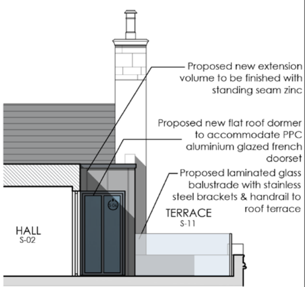
PROPOSED SECTION 8-8 1:100
