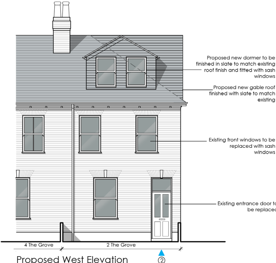
Proposed West Elevation
