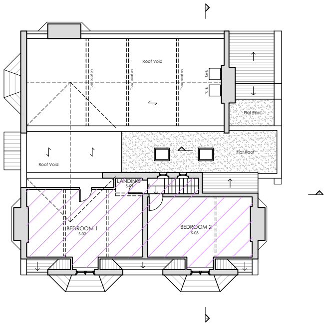
EXISTING SECOND FLOOR PLAN 1:200 GIA = 45.9 sq.m
