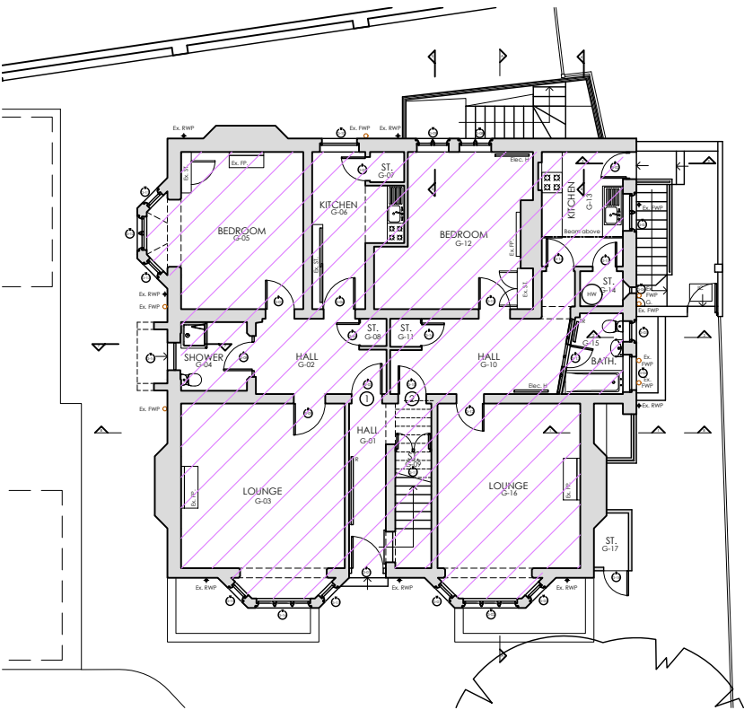
EXISTING GROUND FLOOR PLAN 1:200 GIA = 160.1 sq.m
