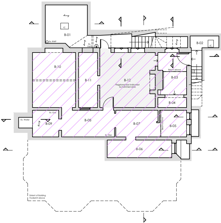
EXISTING BASEMENT FLOOR PLAN 1:200 GIA = 103.1 sq.m
