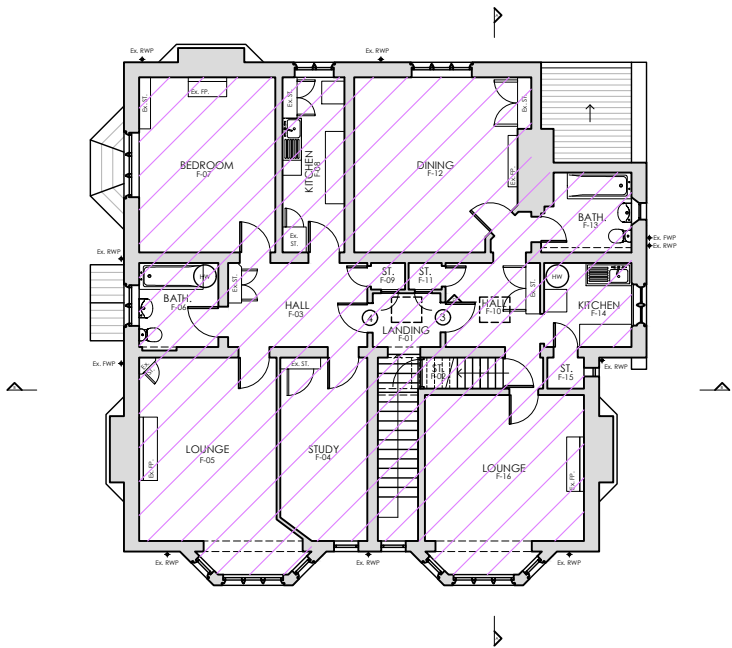
EXISTING FIRST FLOOR PLAN 1:200 GIA = 151.3 sq.m
