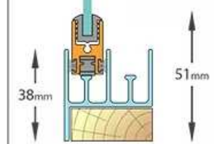
Standard track
