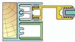
Recessed handle
