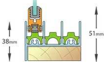
Triple track
