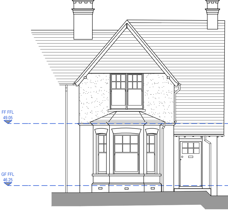
Existing Front Elevation - 1:100 @ A1
