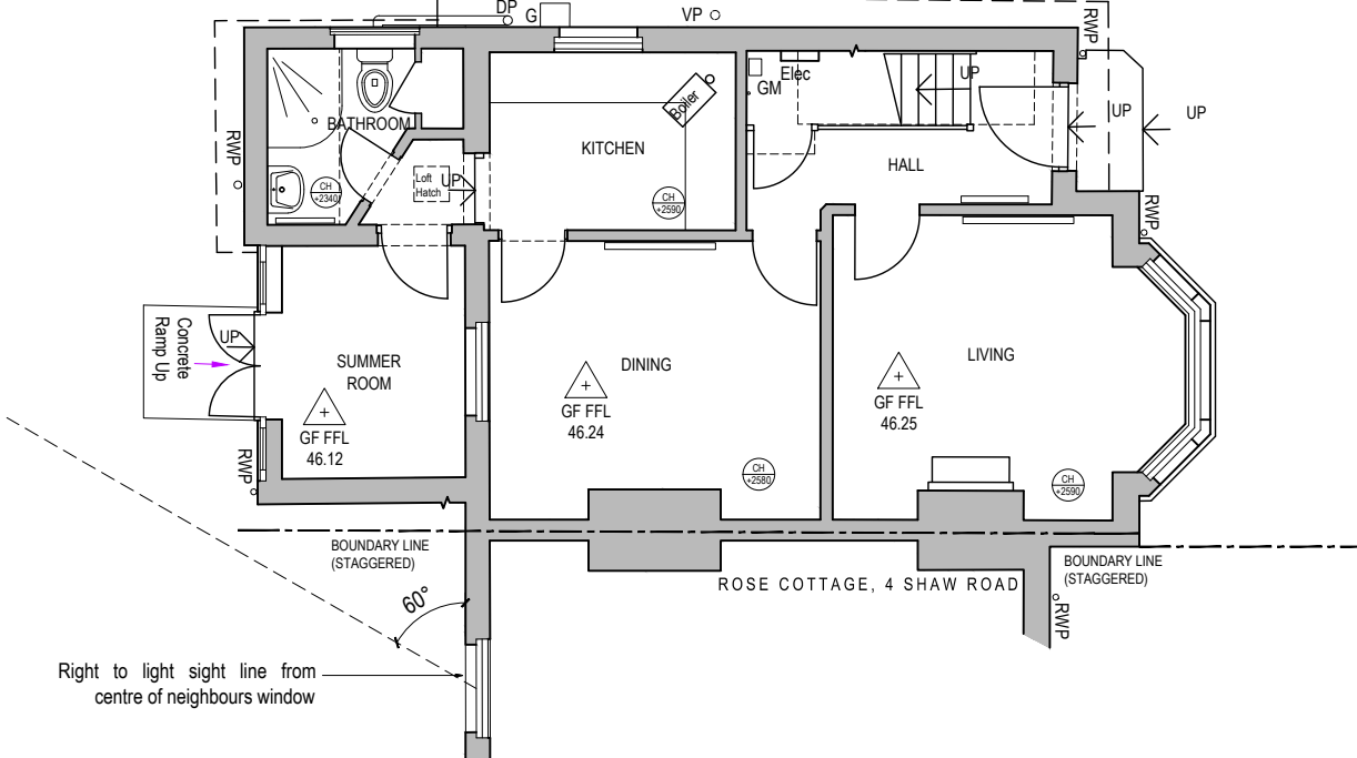
Existing Ground Floor Plan - 1:100 @ A1
