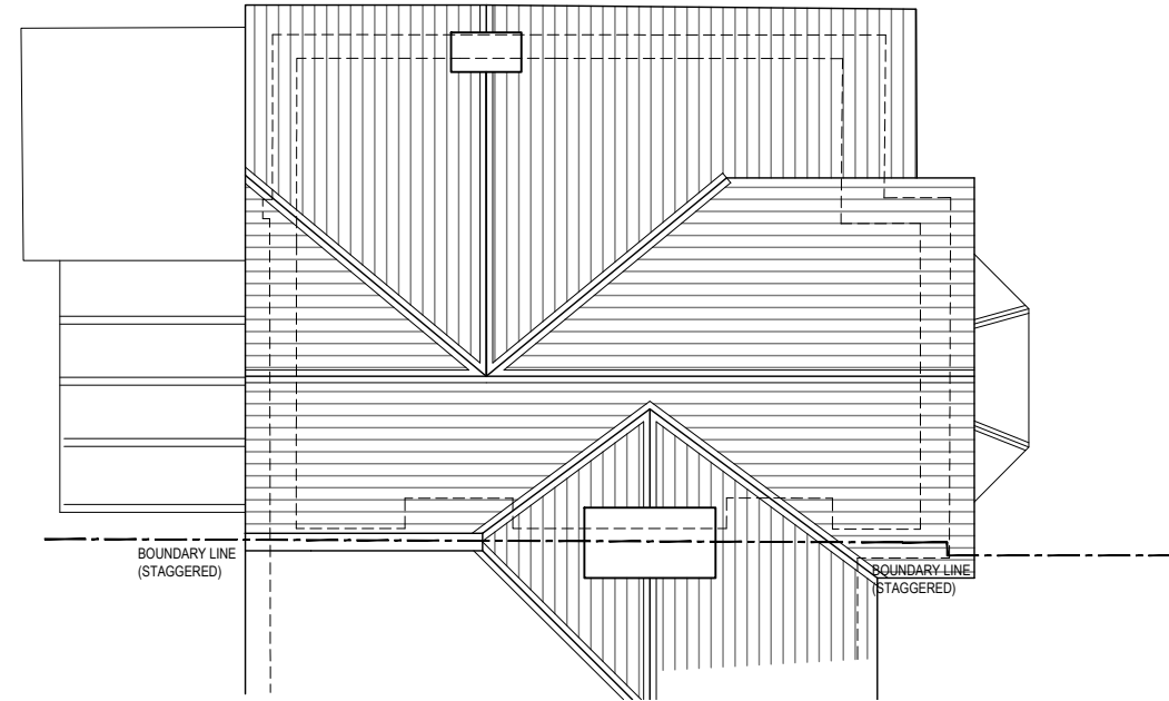
Existing Roof Plan - 1:100 @ A1
