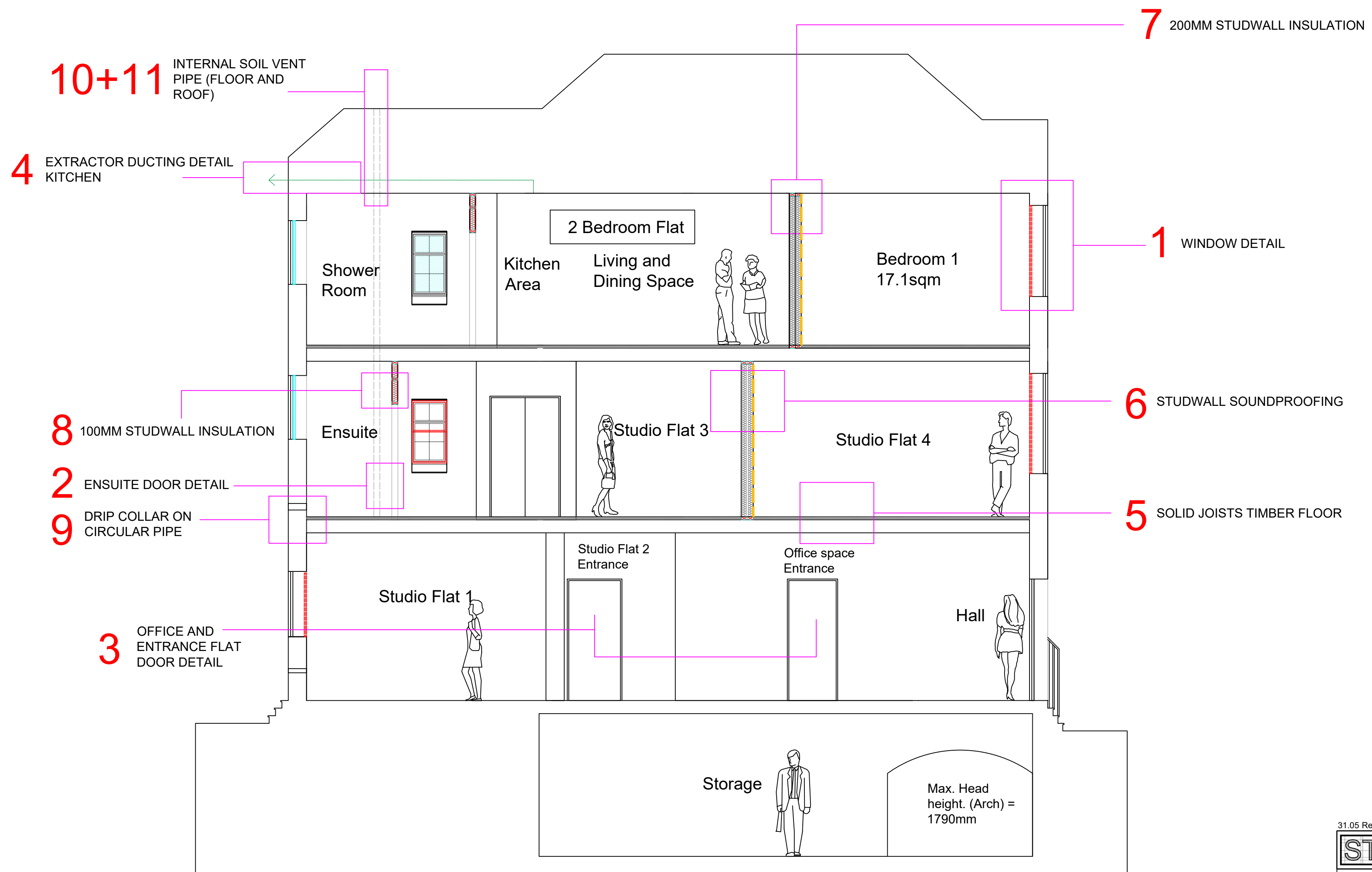
Section AA
