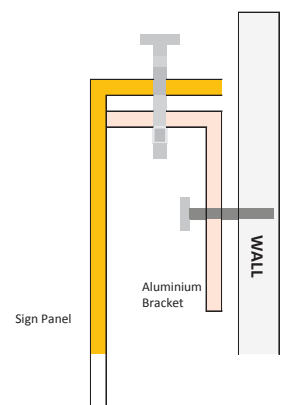
Fixing Method
