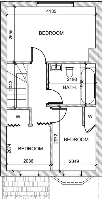
EXISTING FIRST FLOOR PLAN
