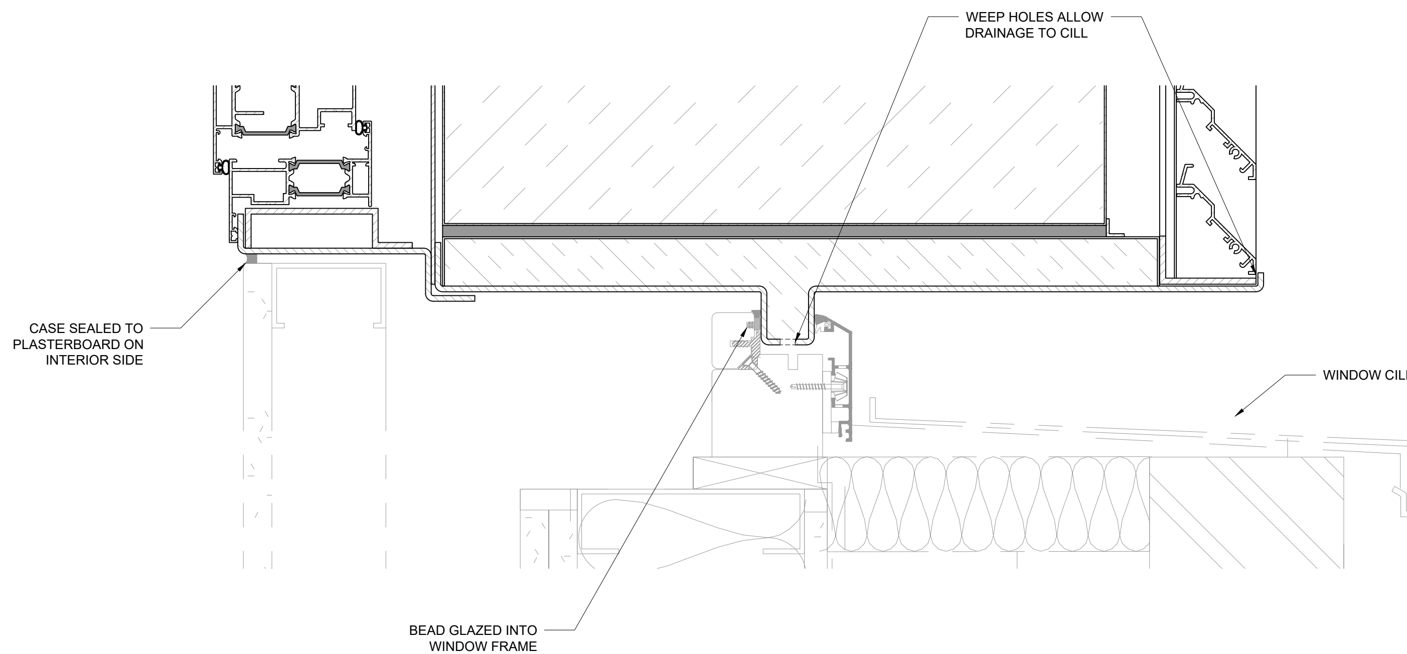
FOOT DETAIL VIEW (1:2)
