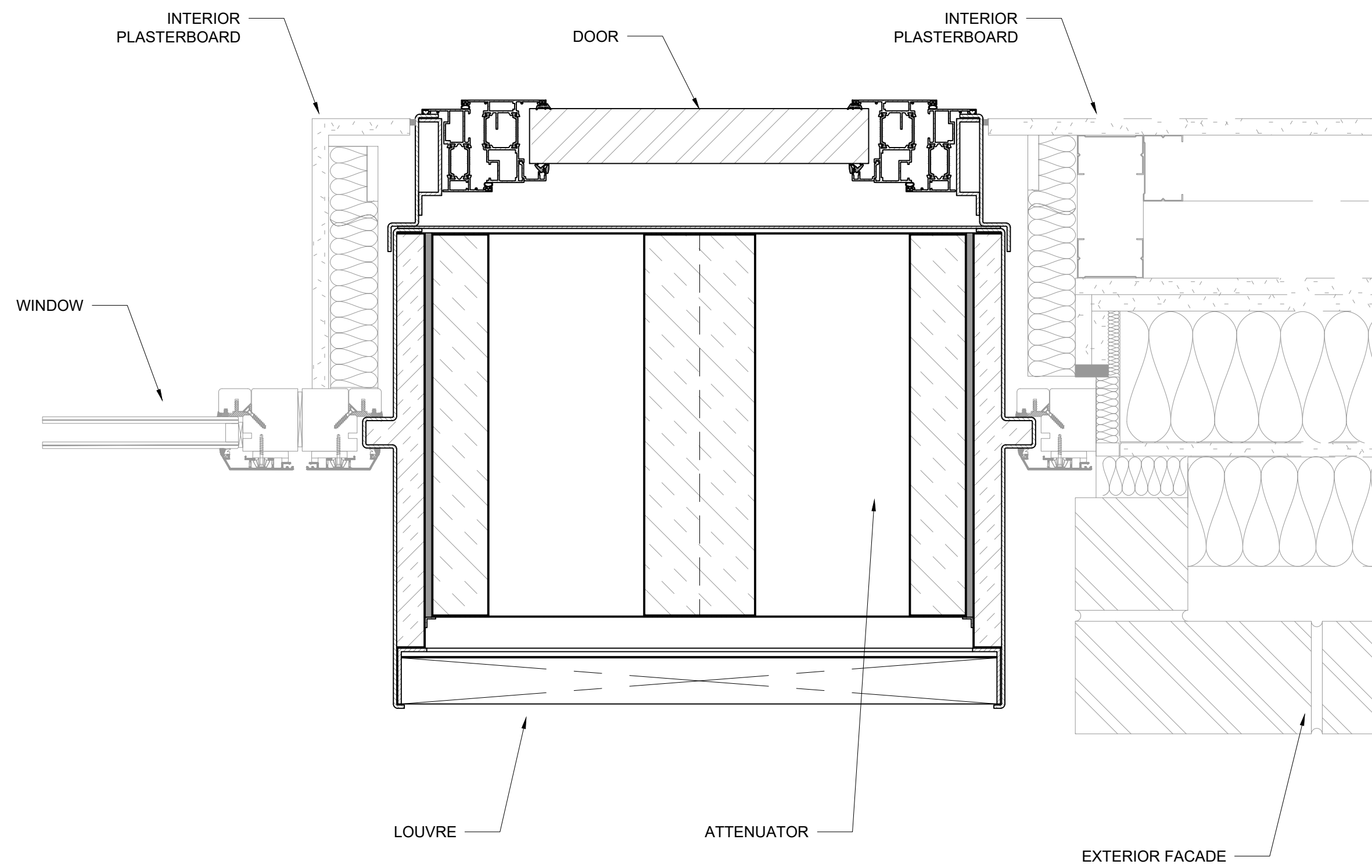
TYPICAL PLAN VIEW
