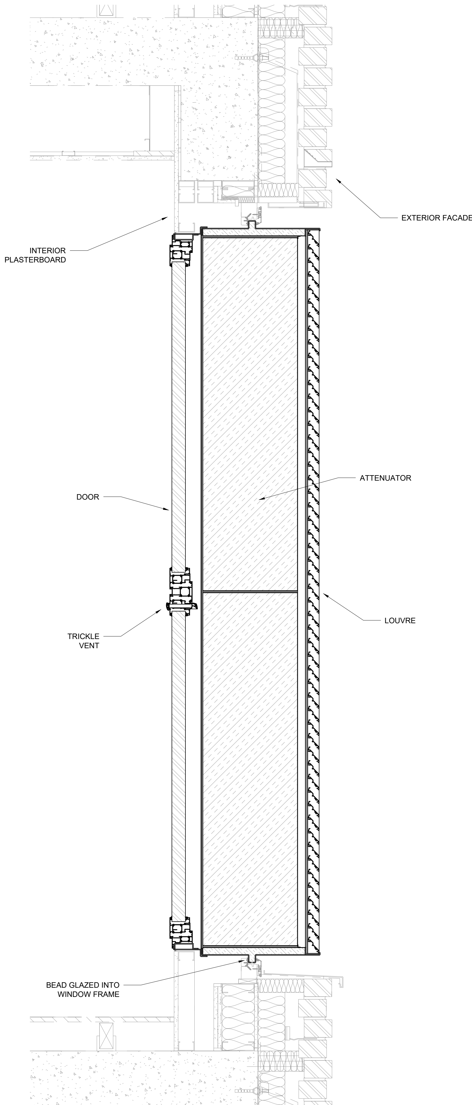
TYPICAL SECTION VIEW
