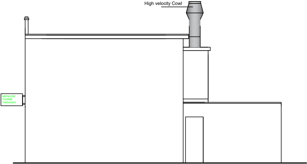
PROPOSED SIDE ELEVATION 1
