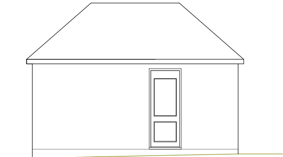
GARAGE NORTH ELEVATION
