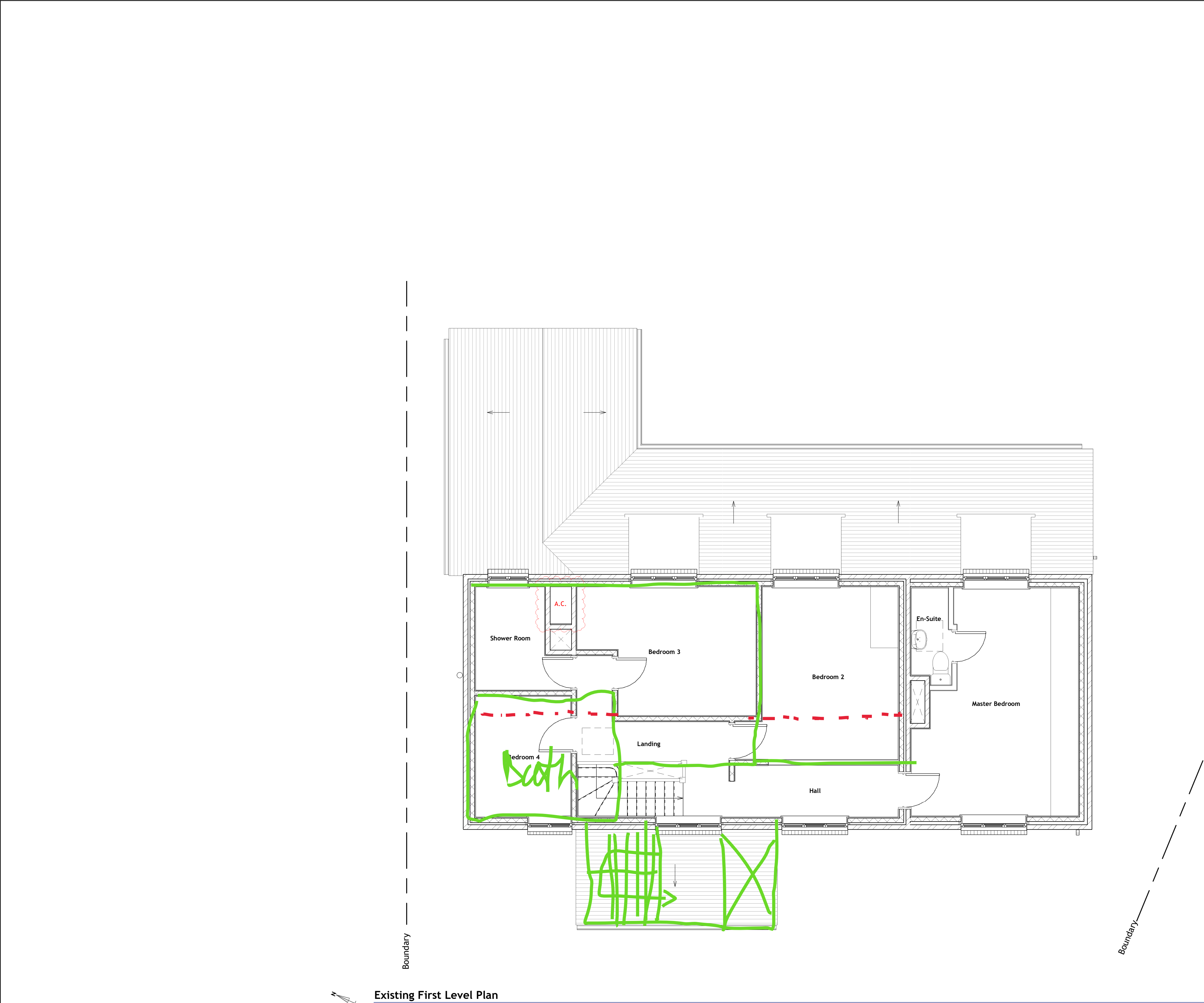
Existing First Level Plan General Arrangement | 01-FFL | Scale 1 : 50
