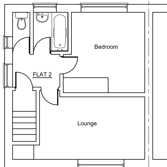
EXISTING 1ST FLOOR PLAN
