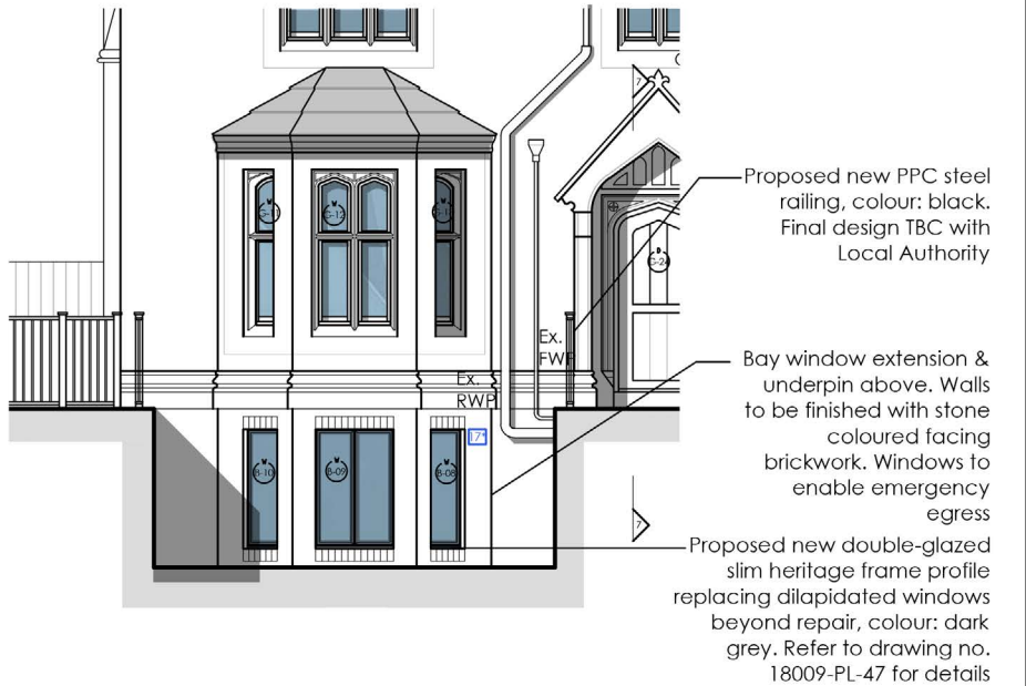
PROPOSED WEST ELEVATION LIGHTWELL 1:100
