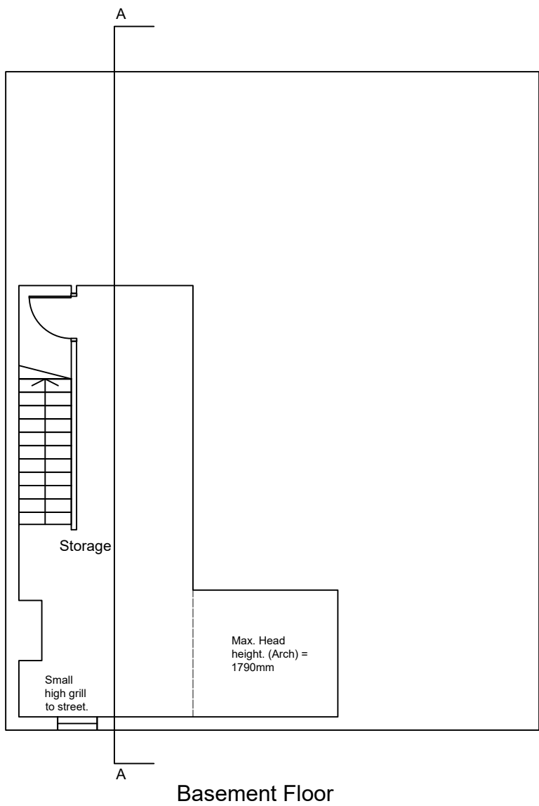
Basement Floor
