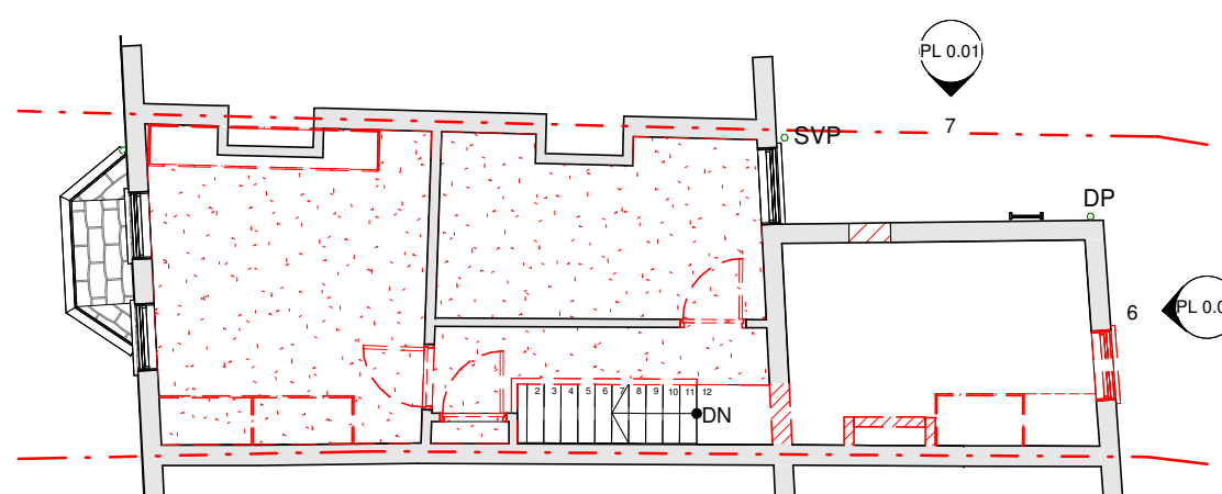
4 First Floor Plan Existing Conditions
