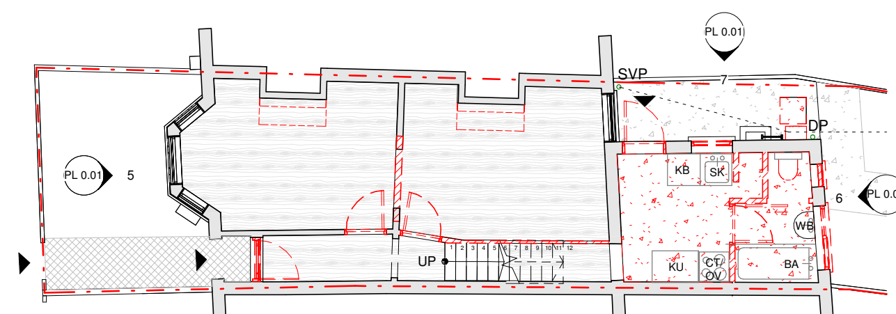
3 Ground Floor Plan Existing Conditions
