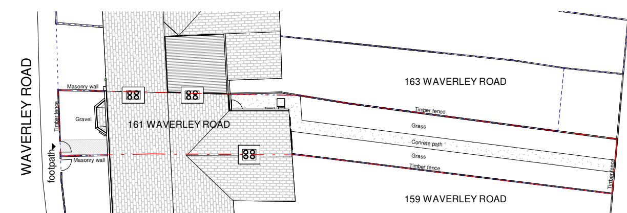
2 Existing Site Plan Existing Conditions
