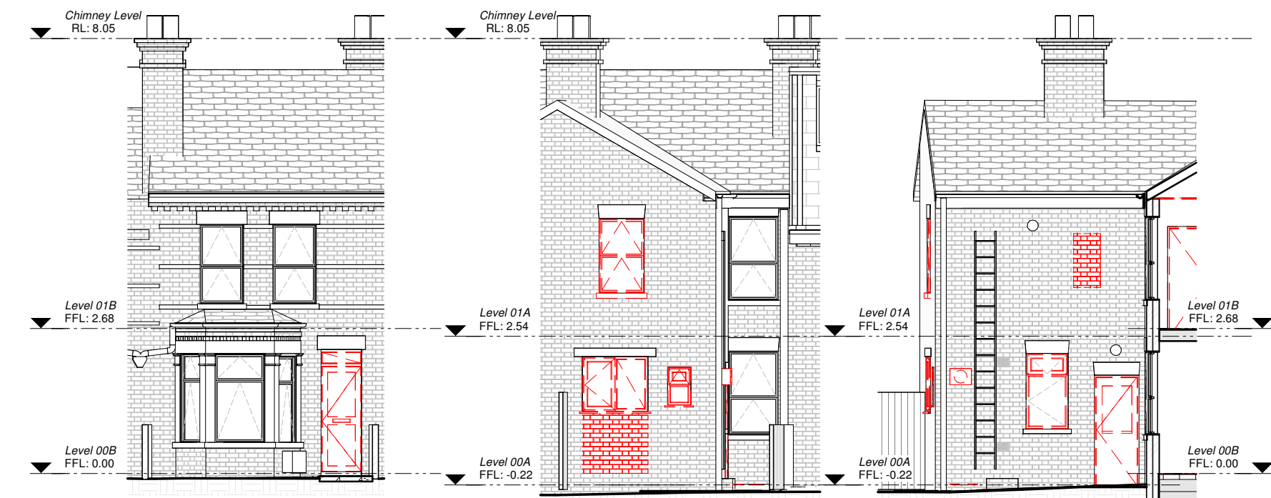
5 Front Elevation Existing Conditions
