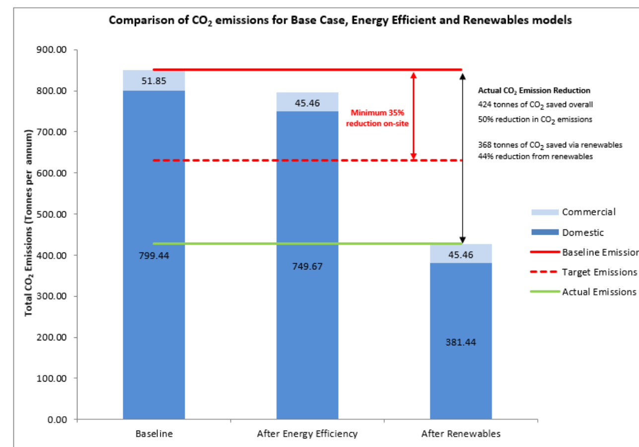
Figure 1: Summary of Regulated CO 2 Emissions
