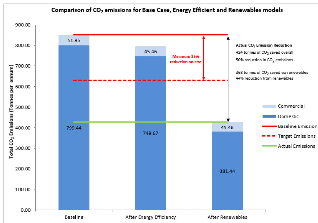
Figure 4: Summary of Regulated CO 2 Emission Savings
