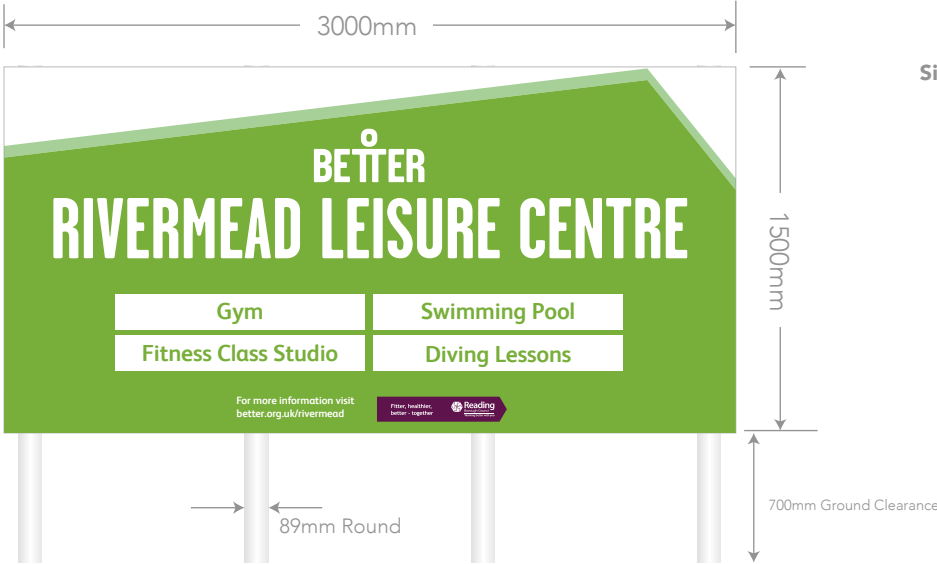
Right Entrance
