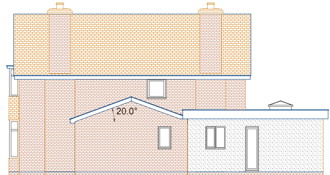
Proposed Side Elevation (R)
