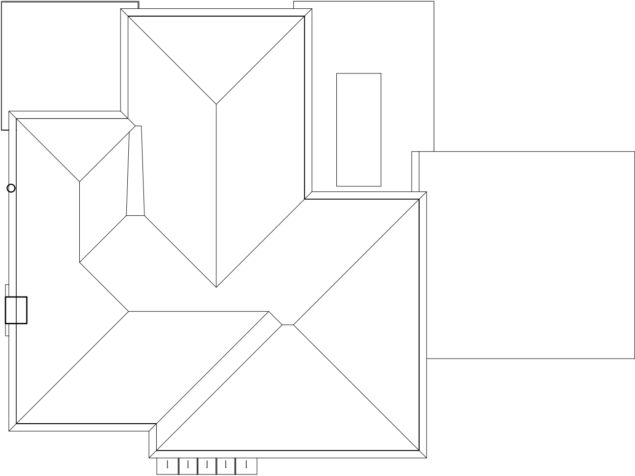
ROOF PLAN
