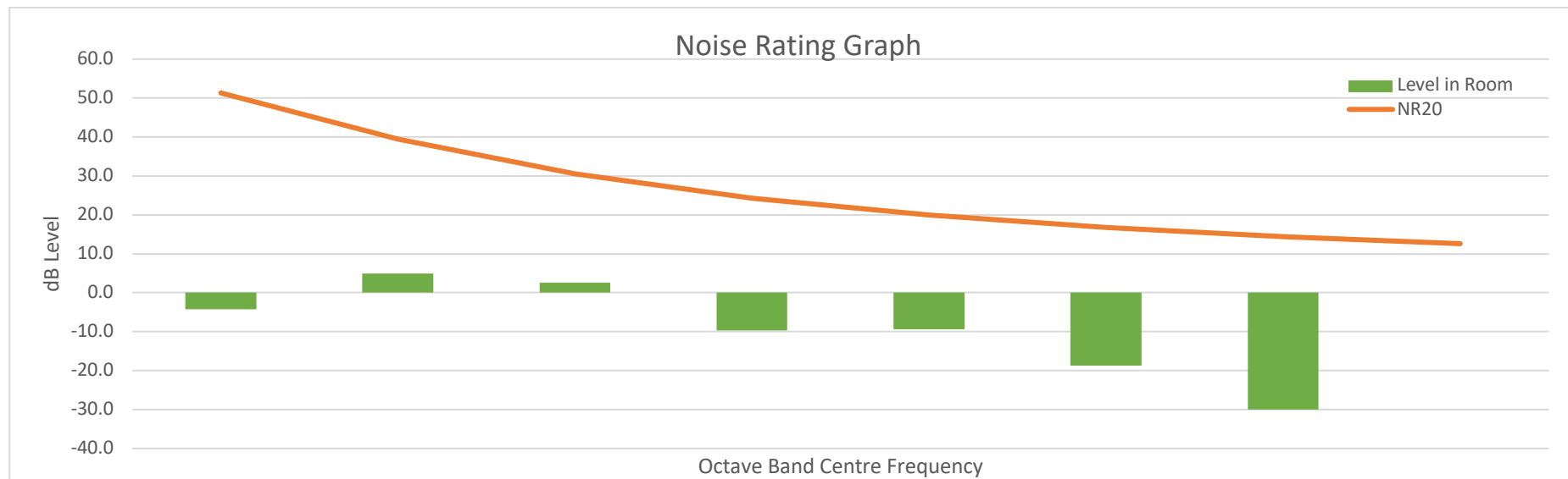
Figure 2: Predicted NR curve against NR20
