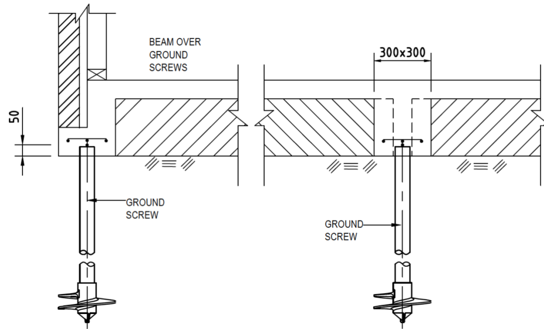
TYPICAL GROUND SCREWS AND BEAM OVER SCREWS DETAIL 25 COCKNEY HILL TILEHURST READING (OUTBUILDING)
