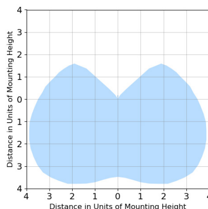
Isoilluminance Plot
