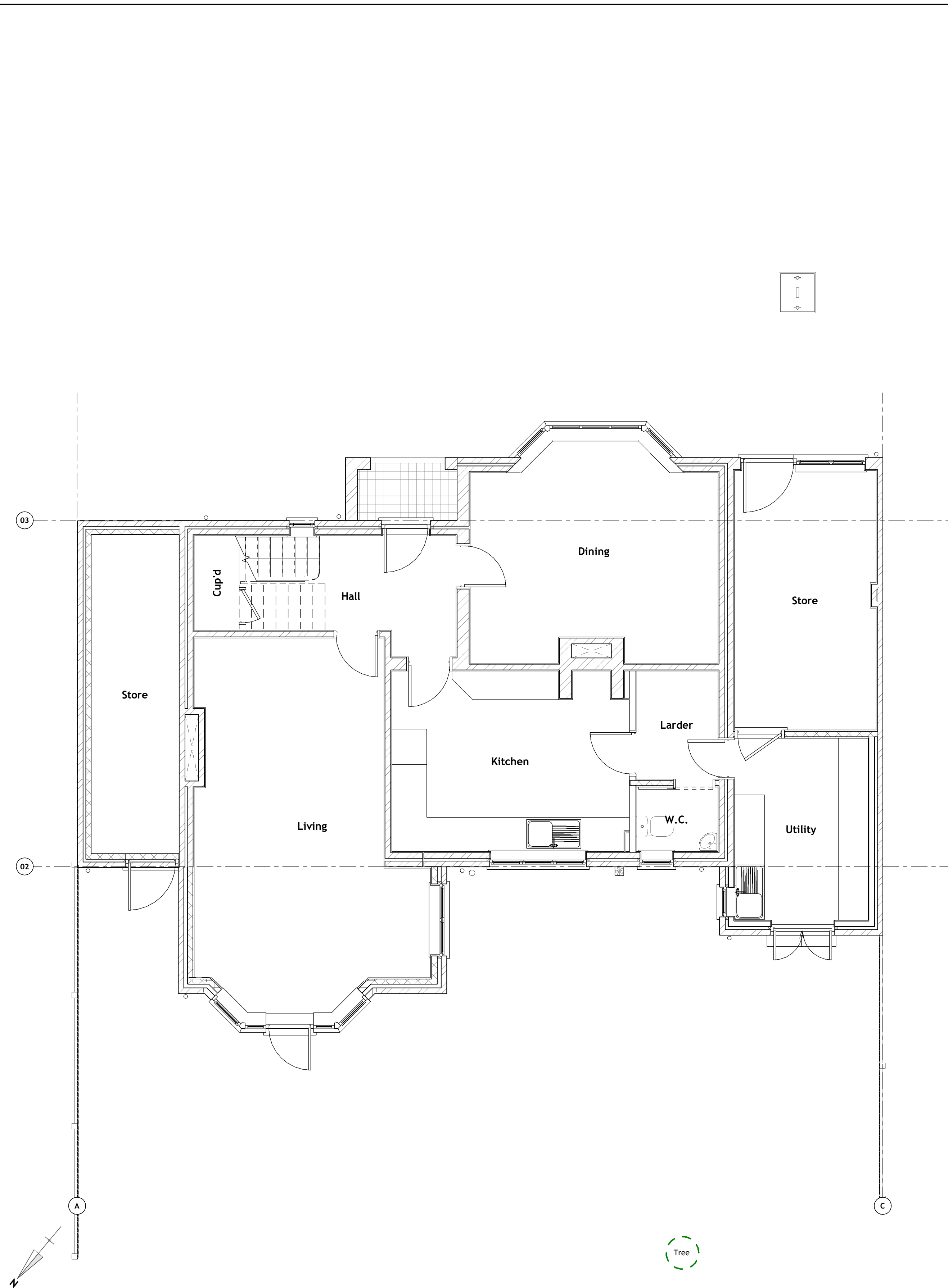
Existing Ground Level Plan General Arrangement | 00-FFL | Scale 1 : 50
