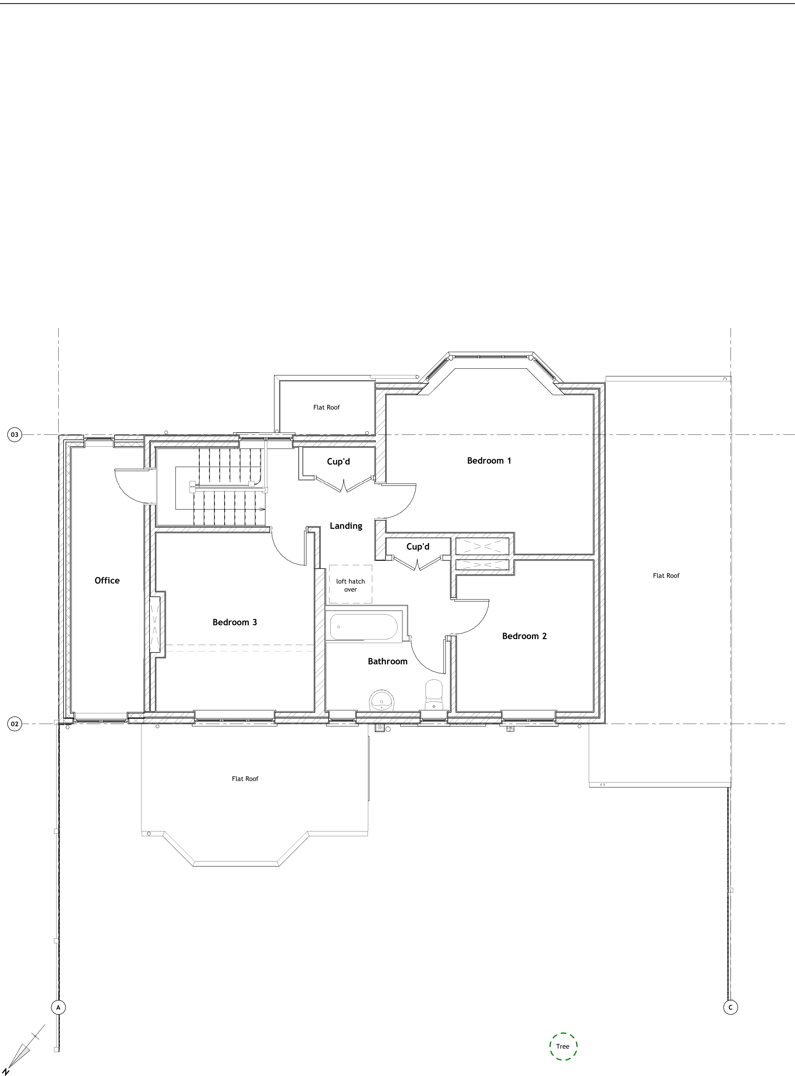
Existing First Level Plan General Arrangement | 01-FFL | Scale 1 : 50
