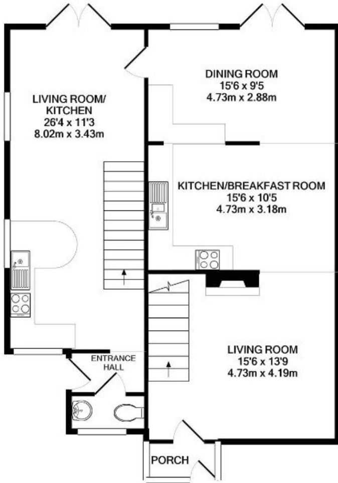
GROUND FLOOR APPROX. FLOOR AREA 877 SQ.FT. (81.5 SQ.M.)
